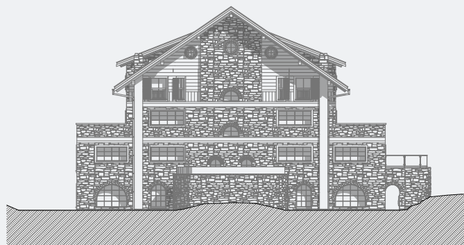
NORTH ELEVATION
